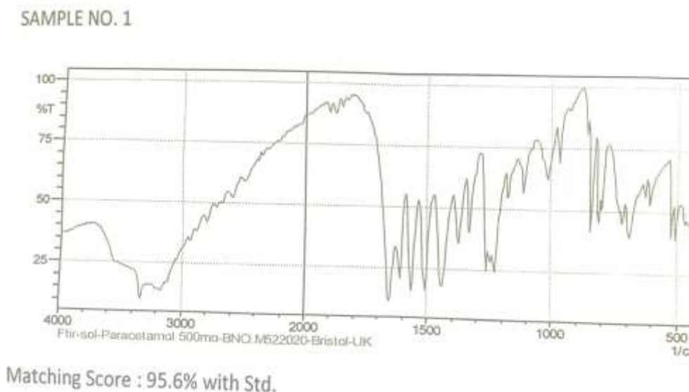
Figure 2. The FTIR spectrum for sample No. 1.
